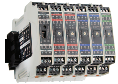
DH2-W Shown with I/O Modules
